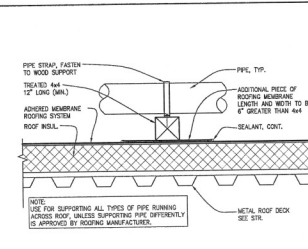
PIPE SUPPORT DETAIL
