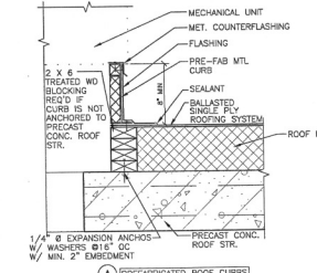
(A) PREFABRICATED ROOF CURBS
