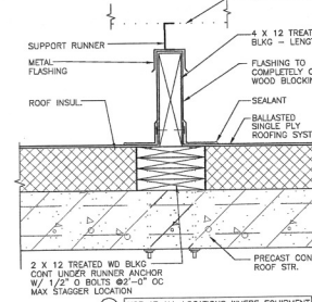
ROOF CURB DETAIL
