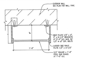
ROOF LADDER PLAN
