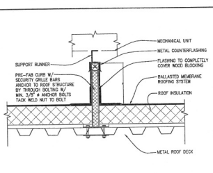
PREFAB. ROOF CURB DETAIL
