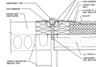
EXPANSION JOINT DETAIL
