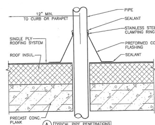
(A) TYPICAL PIPE PENETRATIONS
