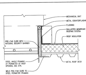
PREFAB. ROOF CURB DETAIL
