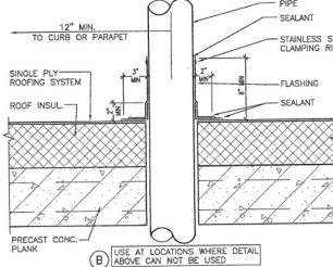
PIPE PENETRATION DETAIL
