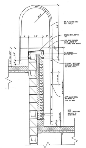
ROOF LADDER SECTION
