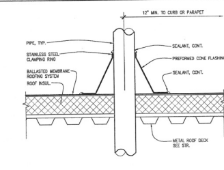
TYP. PIPE PENETRATION
