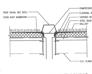
TYPICAL ROOF DRAIN FLASHING
