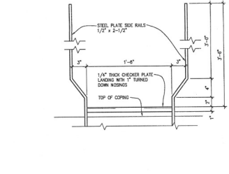
ROOF LADDER PLAN
