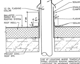
FLUE PIPE PENETRATION DETAIL
