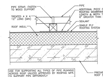
PIPE SUPPORT DETAIL
